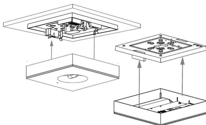
Surface Mounted
